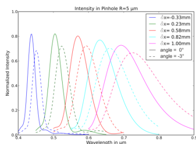
Fig. 3 Simulation of the filtering characteristics
