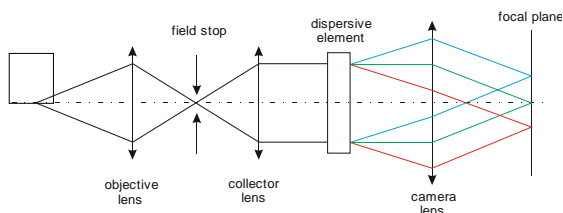
Fig. 1 Principle of a laterally separating hyperspectral imaging system composing the whole picture e.g. by a scanning object or field stop
